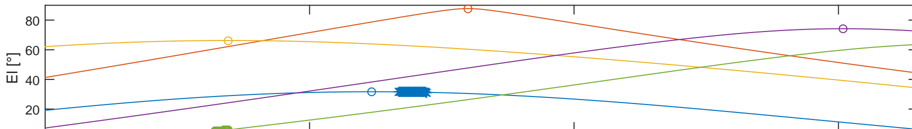
Station: WARK30M
