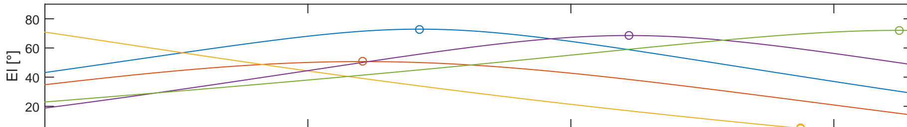
Station: CEDUNA
